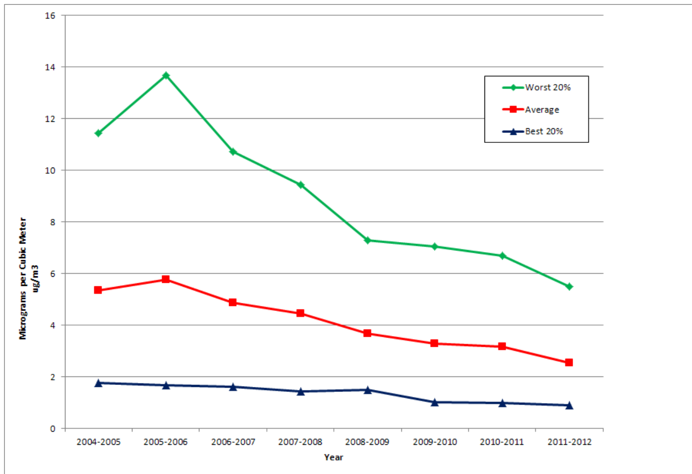
Figure 3 Sulfate Trend Summary** Brigantine, NJ 2004-2012
